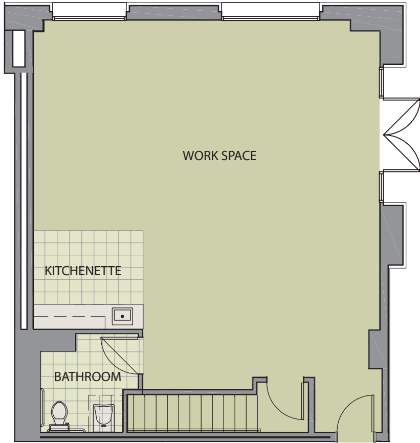
1ST FLOOR
